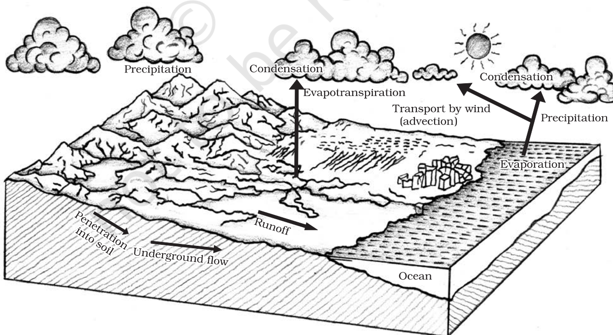
Figure 13.1 : Hydrological Cycle
